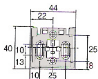
Base du support
