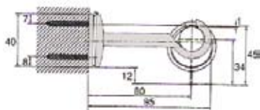
Support mural double
