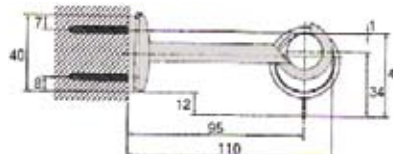
Support mural simple allongé 100 mm
